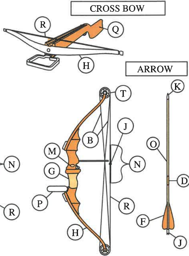
COMPUND BOW
